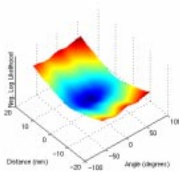
Fig. 6. Samples from the negative log likelihood function over various angles and x-shifts. Note that over this range, the function is very smooth and has one distinct minimum, which in this case occurs 0.86 mm away from the correct alignment.
